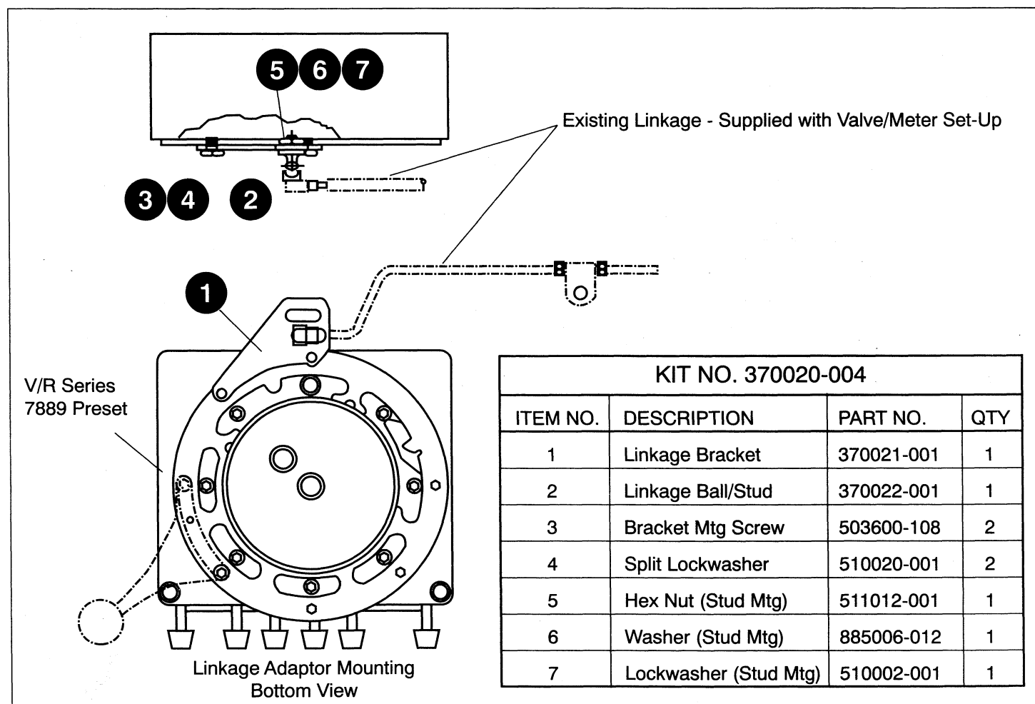
Figure 1. Typical Adaptor Mounting & Kit Parts List
